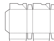
Lock - bottom
